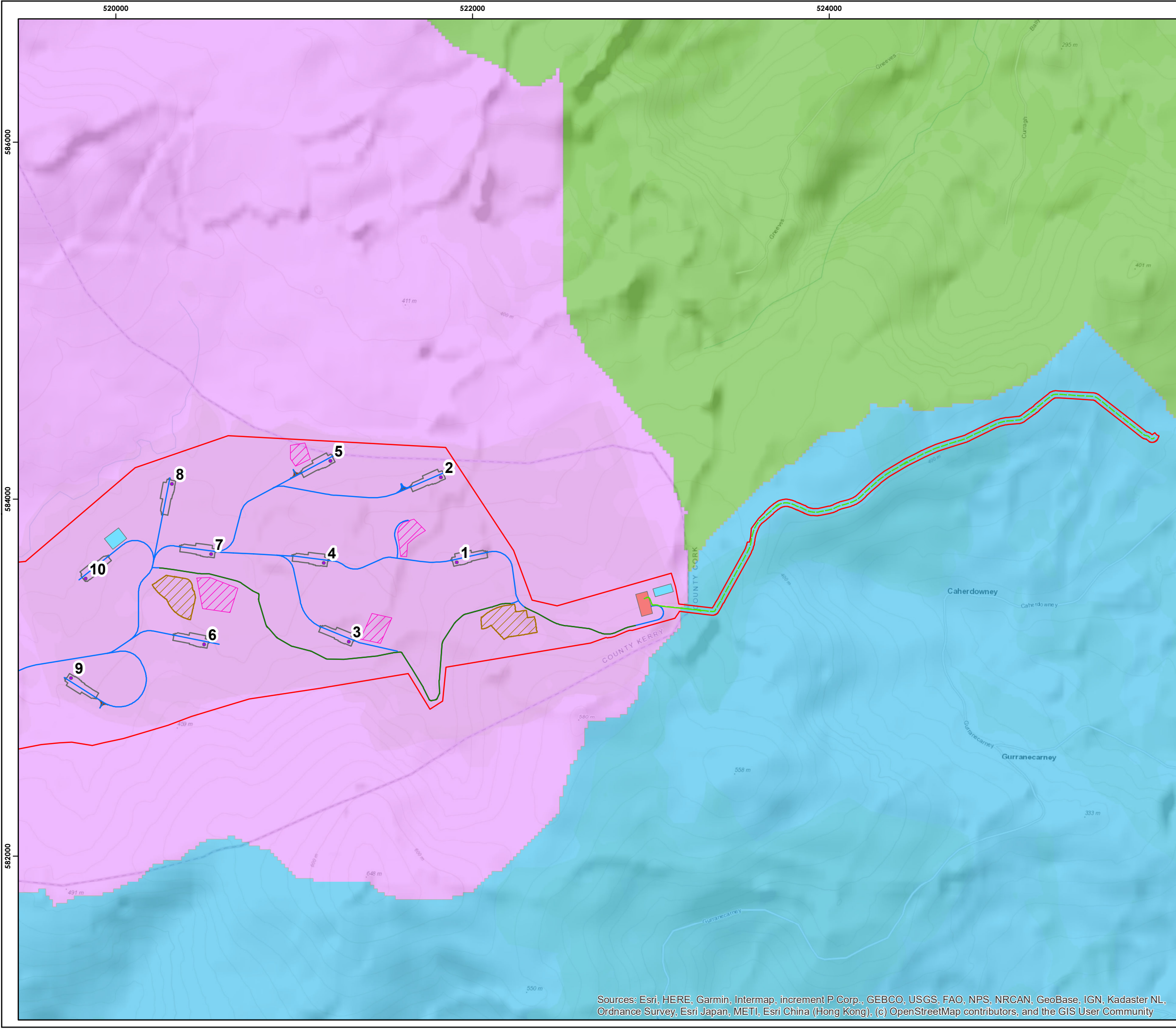
Figure10-4c Groundwater Bodies
